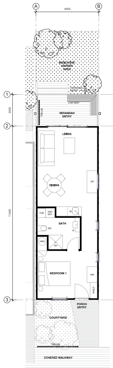
2 L1 - GROUND FLOOR - Unit Plan A1: 1:50
