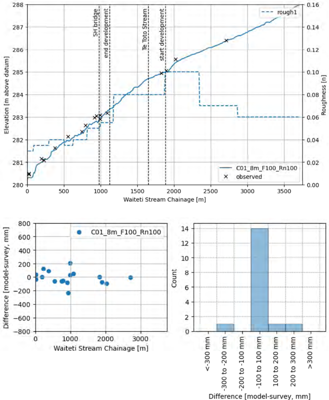
Figure 16: Calibration to the 27/28 April 2018 event, long section (top), differences (model-surveyed) vs chainage (bottom left) and histogram of differences (bottom right)
