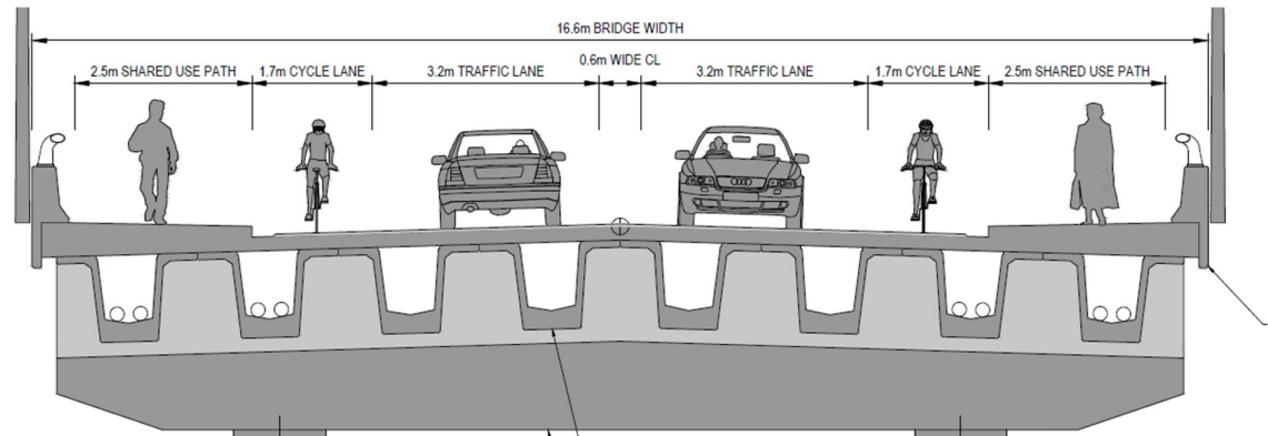
Figure 0-2: Proposed bridge cross section
