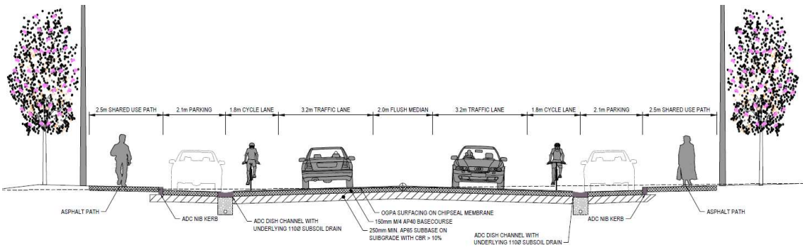
Figure 0-3: Proposed road cross section (where on street parking is provided)
