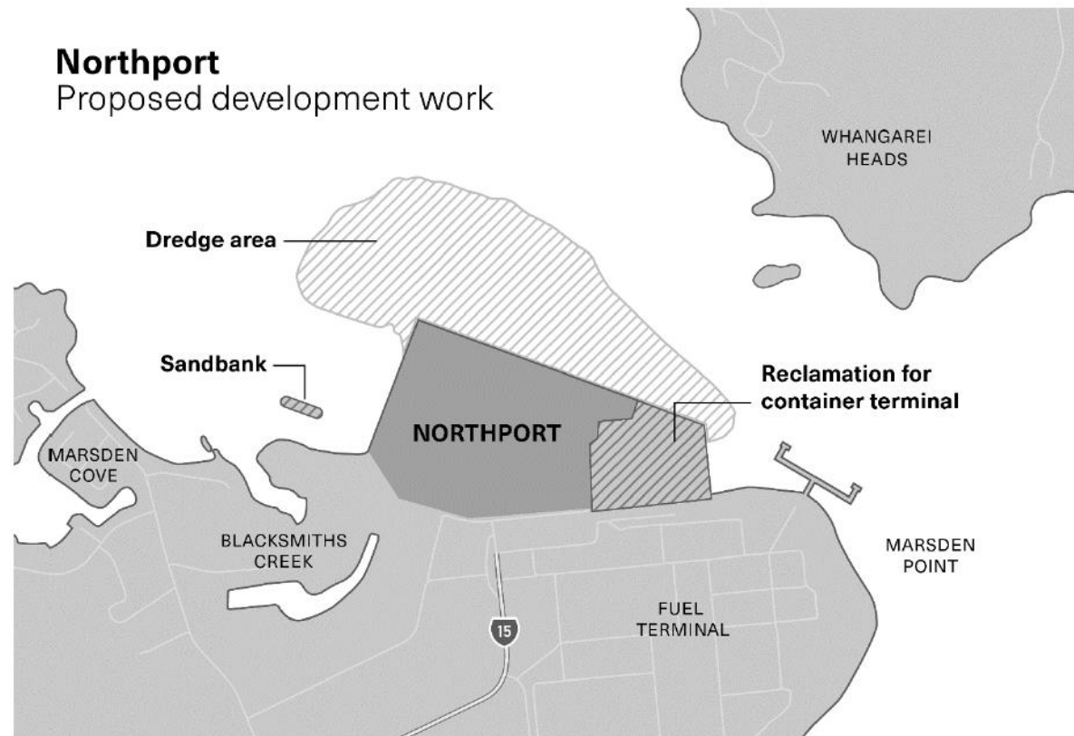
Figure One: Indicative plan showing the general location and fundamentals of the proposal ( the proposed development is hatched )
