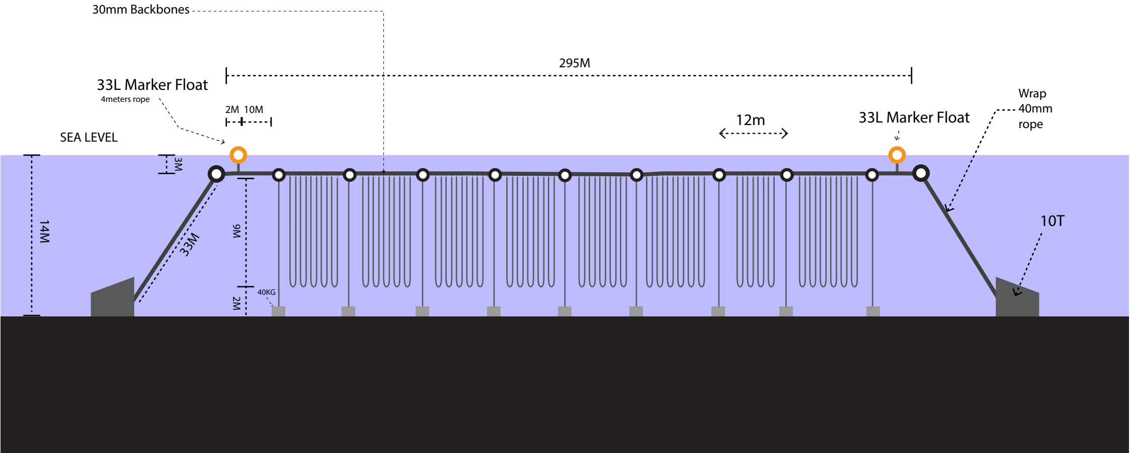
SECTION DRAWING DRAWN BY: ZOE REDWOOD
