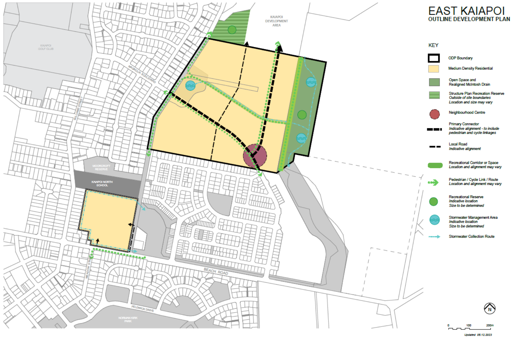
Figure 7: Proposed Outline Development Plan
