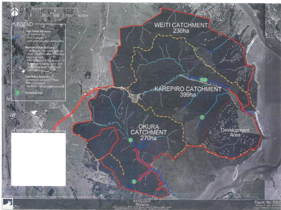
Diagram 3: Weiti catchments
