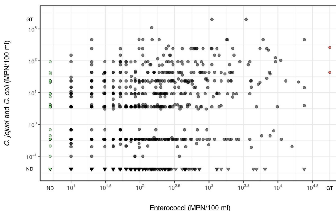
Figure 20: Comparison of Campylobacter ( C. jejuni and C. coli ) and enterococci concentrations in freshwater samples.
