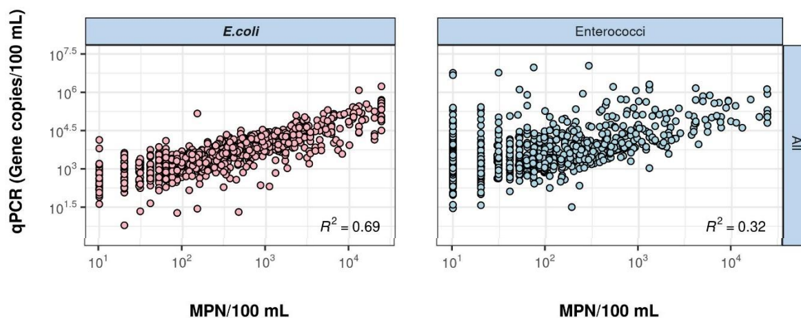
Figure 4: E. coli and enterococci concentrations by culture and qPCR
