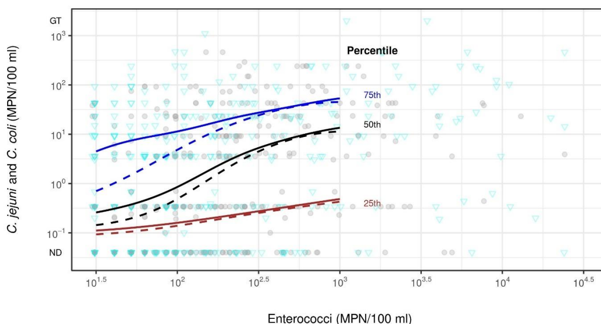
Figure 21: Comparison of Campylobacter ( C. jejuni and C. coli ) concentrations with enterococci concentrations in freshwater samples during (circles) and outside (triangles) the bathing season. Solid lines are the quantile regression estimates using all the data and the dashed lines are the quantile estimates based on data collected during the bathing season (31 October to 31 March).
