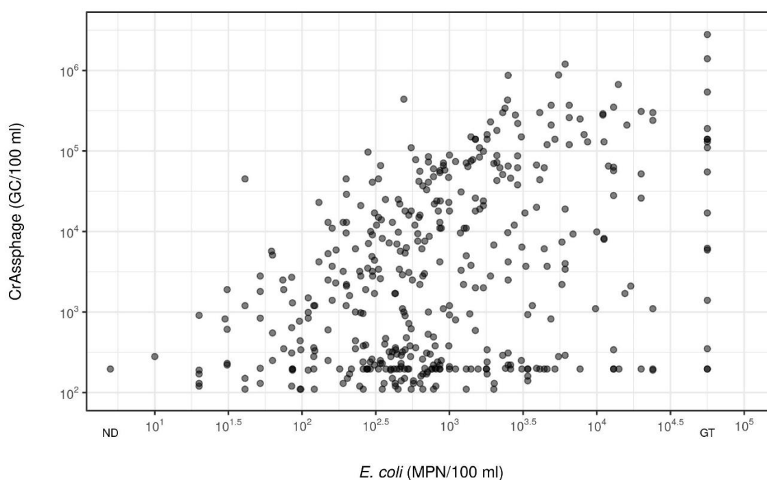
Figure 36 Scatterplot of CrAssphage concentration (GC/100ml) compared with E. coli (MPN/100ml)
