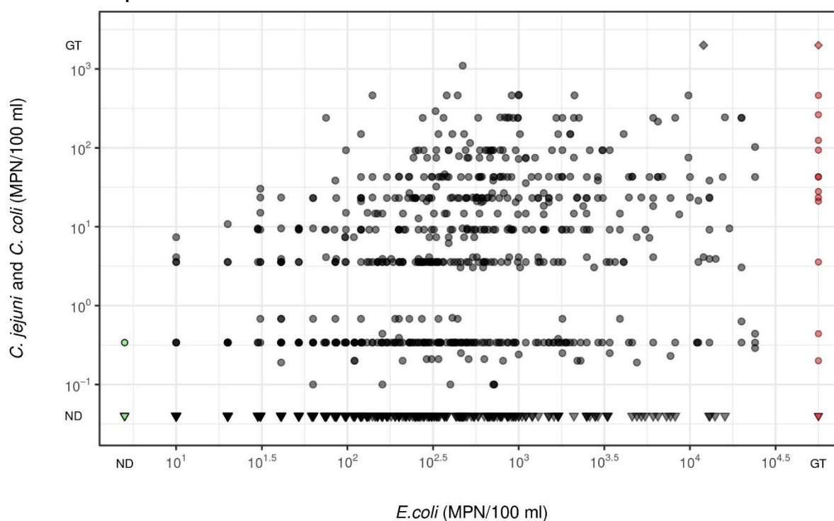
Figure 17: Comparison of Campylobacter (combined C. jejuni and C. coli ) and E. coli concentrations in freshwater samples.
