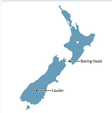
GCOS Figure 1: Key atmospheric constituent climate sites
