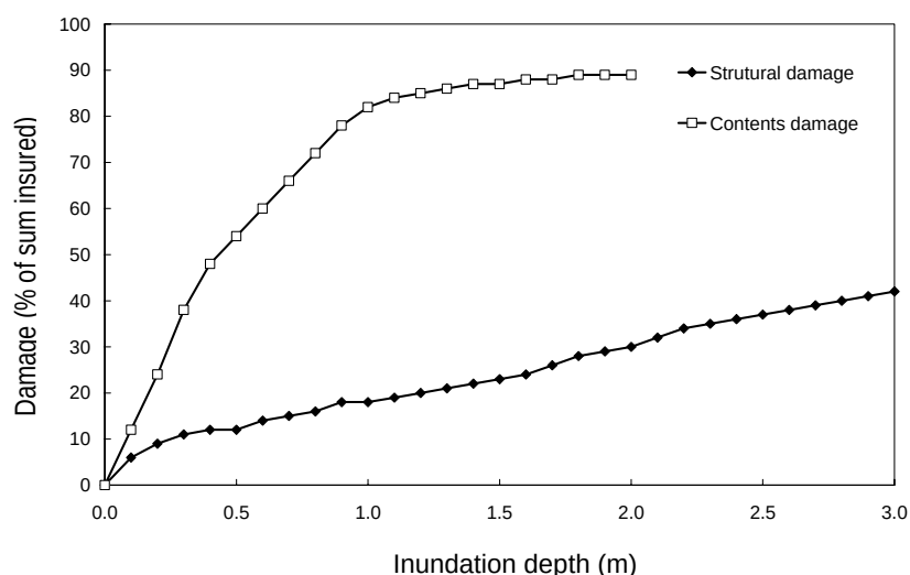
Figure 1 Risk Frontiers depth-damage curve
