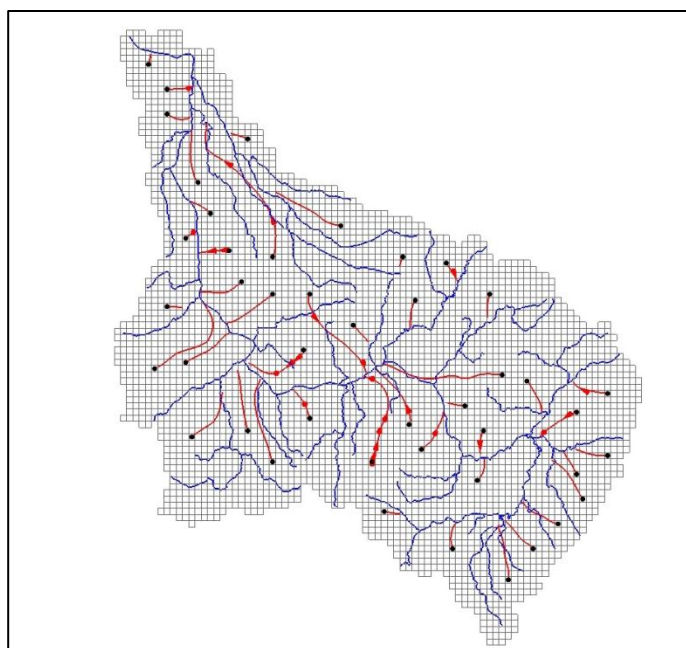
Figure 4: Selected simulated water travel paths.
