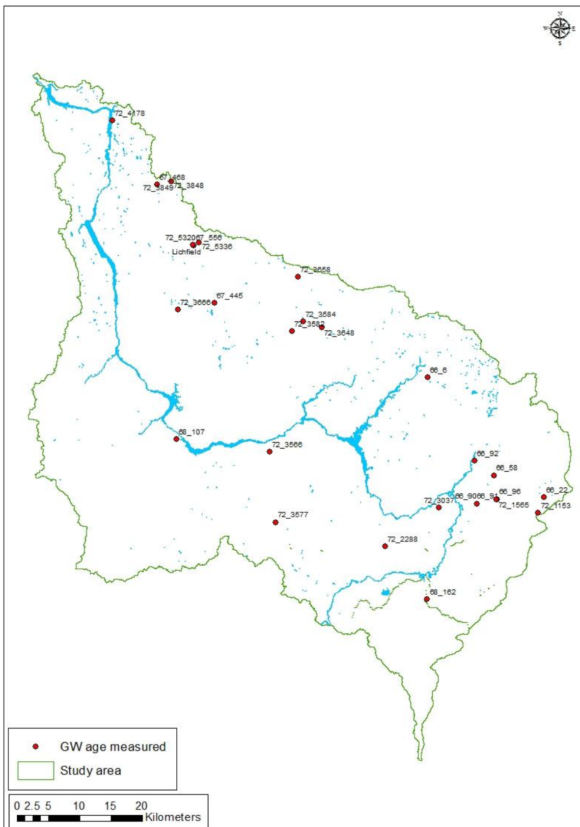
Figure 8: Bore locations where groundwater age is measured.
