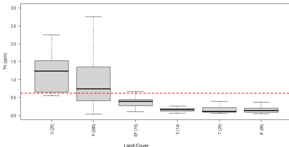
Figure 11: Median TN concentrations (2003–2007) grouped by REC Land-cover categories. See footnote to Figure 2 for explanation of the box plots. The ANZECC trigger values for TN for lowland and upland sites are 0.614 (indicated on the box plot) and 0.295 ppm respectively.
