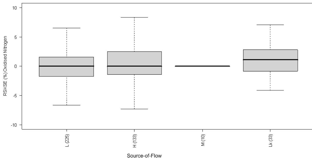
Figure 14: RSKSE values for \text{NO}_x\text{-N} grouped by REC Source-of-flow categories for 1998–2007. See footnote to Figure 2 for explanation of the box plots.
