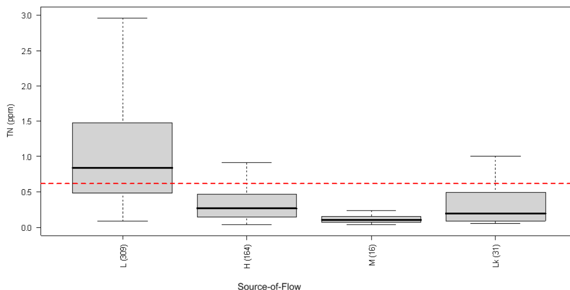
Figure 9: Median TN concentrations (2003–2007) grouped by REC Source-of-flow categories. See footnote to Figure 2 for explanation of the box plots. The ANZECC trigger values for TN for lowland and upland sites are 0.614 (indicated on the box plot) and 0.295 ppm respectively.
