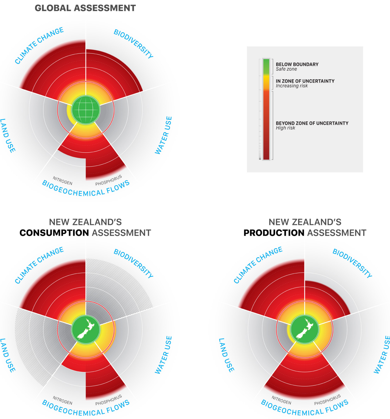
Figure 21: The radial plots show global (top) and national (bottom) status of five planetary boundaries on a normalised scale. New Zealand exceeds its “fair share” of the global safe operating space for most production-based (territorial) and consumption-based boundaries. The safe zone is depicted in the centre, where the edge of the green circle is the normalised boundary (= 1). After boundary transgression is a zone of increasing but uncertain risks (= 1 – 2). Beyond this is a zone of high risk, depicted by the red line (= 2), which equates to boundary transgression by a factor of 2. From the red line outward, factors of transgression continue approximately according to the white lines. The scale is capped at a factor of 15. Note that phosphorus on the production side is at 55 times transgression and therefore goes off the chart.
