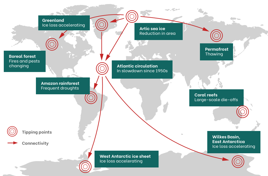
Figure 6: Currently active tipping elements in the Earth system. In 2008, 15 tipping elements were identified. In 2019, empirical evidence indicates many of these potential tipping elements are changing at unprecedented speeds and scales. Some may recently have crossed tipping points, for example, the West Antarctic Ice Sheet. Several tipping elements are connected. 12
