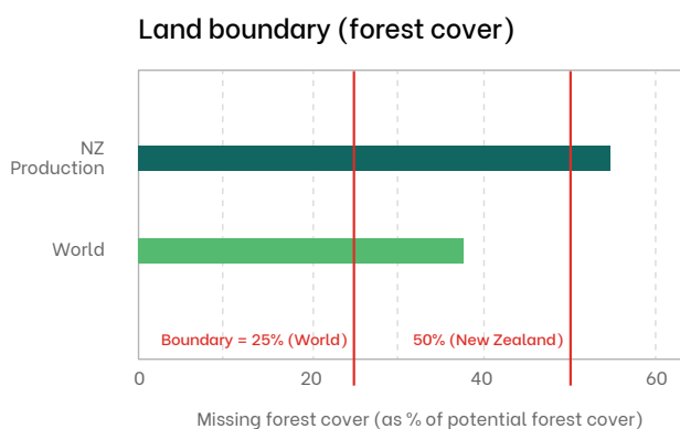
Figure 14: Land boundary based on forest cover (territorial/production only), with global average for comparison. Based on original forest extent, the global boundary is placed at 25% missing, and New Zealand's biome boundary is placed at 50% missing.
